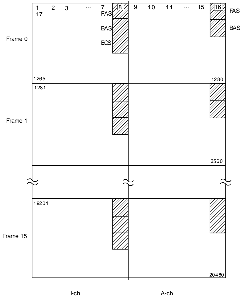
Figure B.1: Bit numbering and unenciphered bits in a multiframe for 2 × B channel
